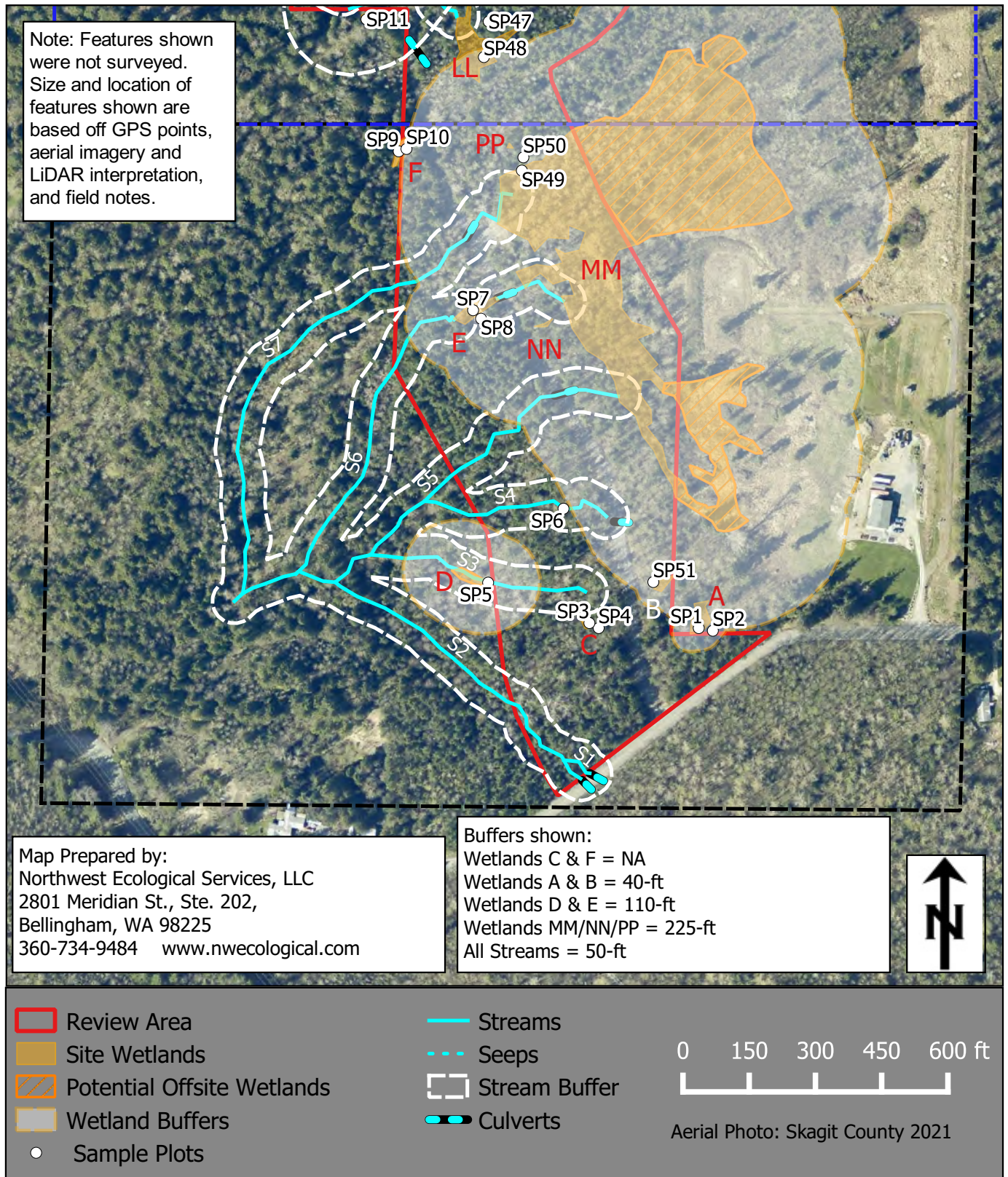
E COLOGICAL NORTHWEST Wetland/ Stream Detail Map (Area 1) Grip Road Gravel Mine Impact Assessment & Mitigation Plan Figure 5 DEC 2021
